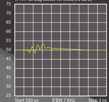
7601+7601-03 (LIN MAG) Tr 4 s11 Lin Mag 5.000U/ Ref 50.00u [F2 Gat zr]
