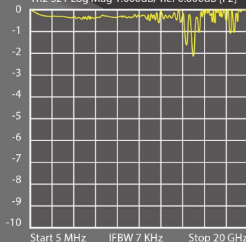
7601+7601-02 (S21MAX) TR2 S21 Log Mag 1.000dB/ Ref 0.000dB [F2]
