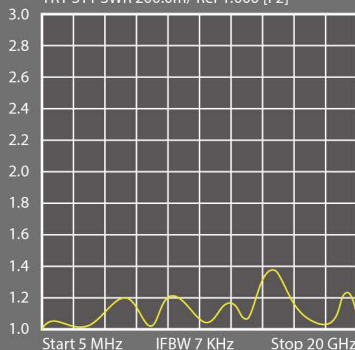
7601+7601-03 (S11MAX) TR1 S11 SWR 200.0m/ Ref 1.000 [F2]
